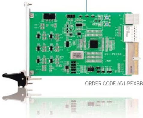
CompactPCI Express Bridge Board
