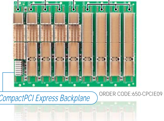
Hybrid Peripheral Slot CPCI Legacy Peripheral Slot(4Slot) System Slot Bridge Slot
